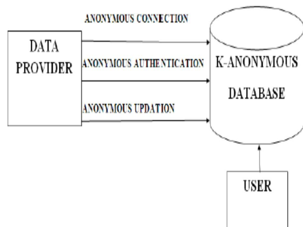
Figure 1: Anonymous Database
