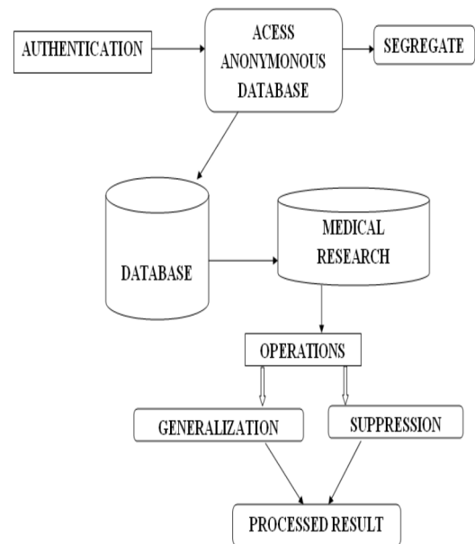
Figure 3: System Architecture
